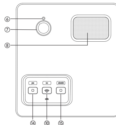
Quinta MU 21 V Delegate Microphone Unit
