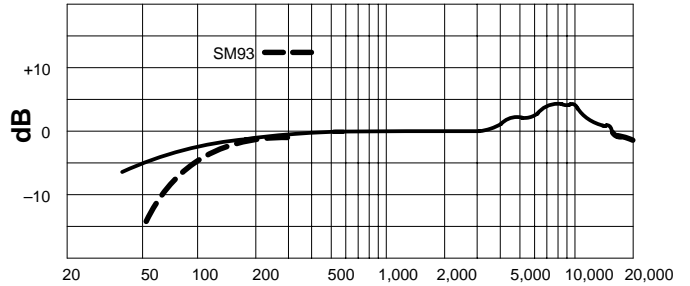
TYPICAL FREQUENCY RESPONSE FIGURE 4
